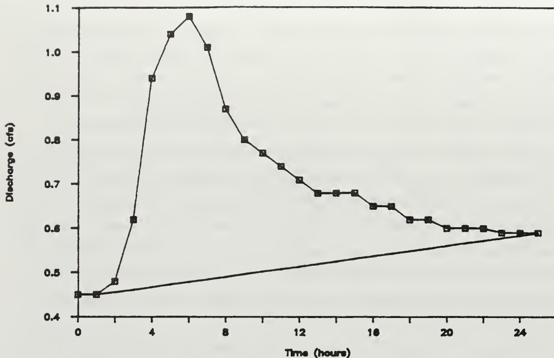
Figure 1. Hydrograph with visually separated baseflow for derivation of a unit hydrograph and determination of T_r/T_p ratio for Deer Creek, Oregon Coast Range.
